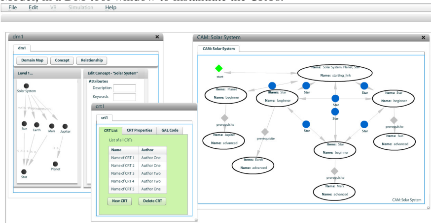
Fig. 1. Authoring tool
